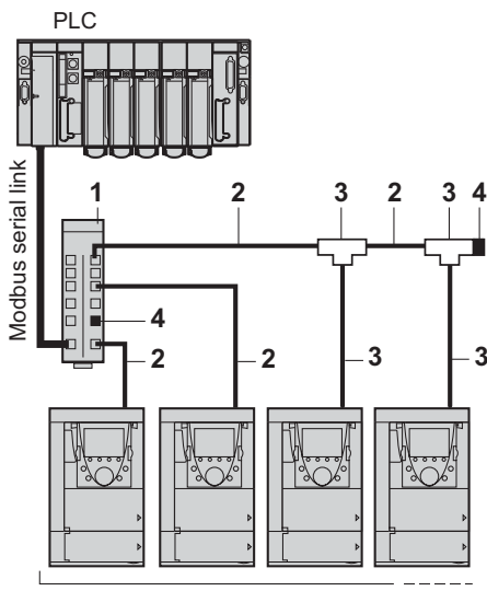
Example of Modbus diagram, connection via splitter boxes and RJ45 connectors
