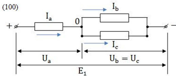
Fig.3 Equivalent circuit for (100) combination
