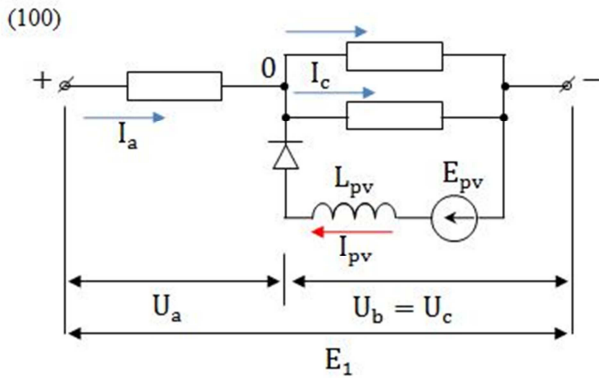
Fig.5 Equivalent circuit with additional power supply
