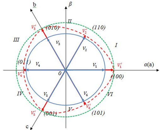
Fig.7 Voltage vector diagram for all sectors
