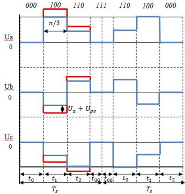
Fig.6 Phase voltage diagram with an additional source
