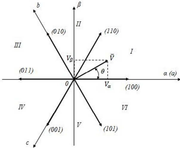
Fig.2. Voltage vector diagram
